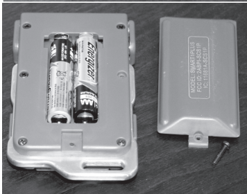
Above: The SMART1+™ transmitter is compact and easy to operate. Inset top: Patent-pending flip-style cover has the SMART1+™ insignia. At bottom: Runs on AAA batteries for longer life; back removes with a single screw for easier battery replacement.
